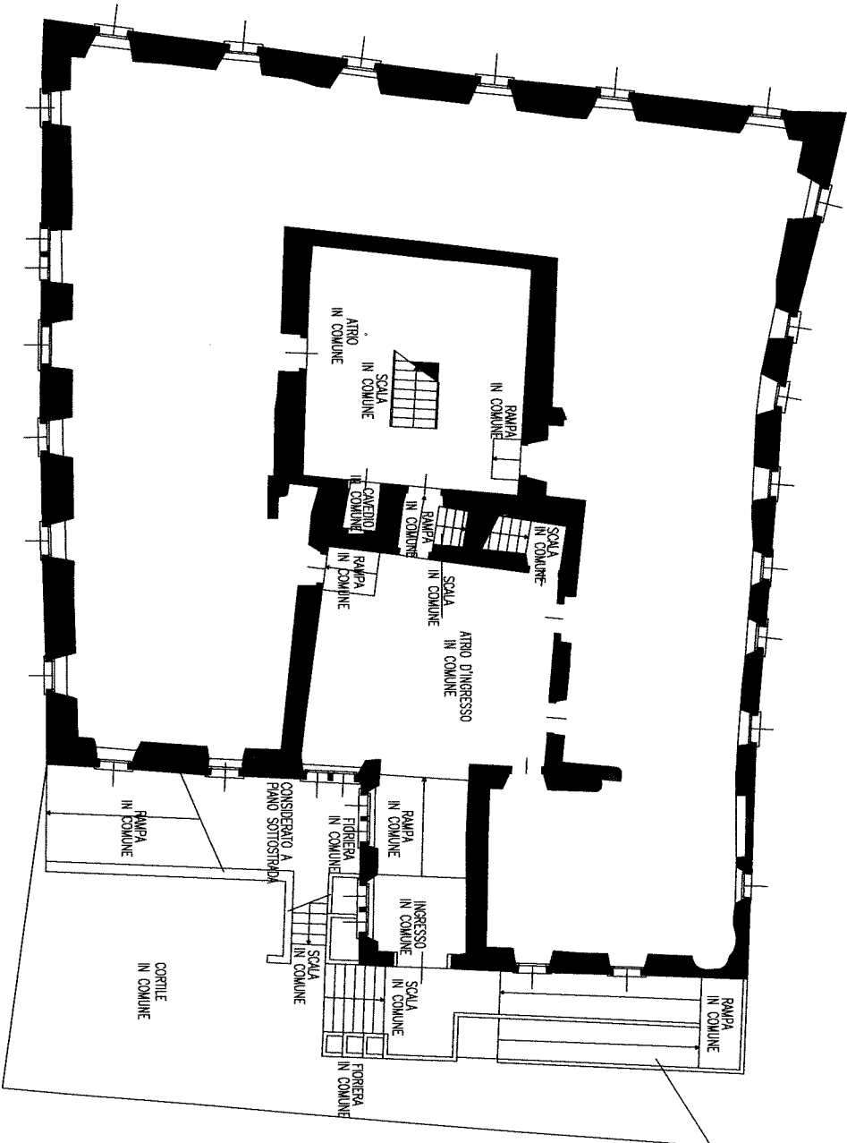
PIANO TERRA
